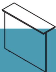
DMC 070 700 x 400 x 1200 DMC 120 1200 x 400 x 1200 DMC 140 1400 x 400 x 1200 DMC 160 1600 x 400 x 1200
