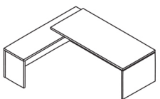
TCT 1820 L/R 1800 x 2000 x 750 TCT 2020 L/R 2000 x 2000 x 750 TCT 2220 L/R 2200 x 2000 x 750
